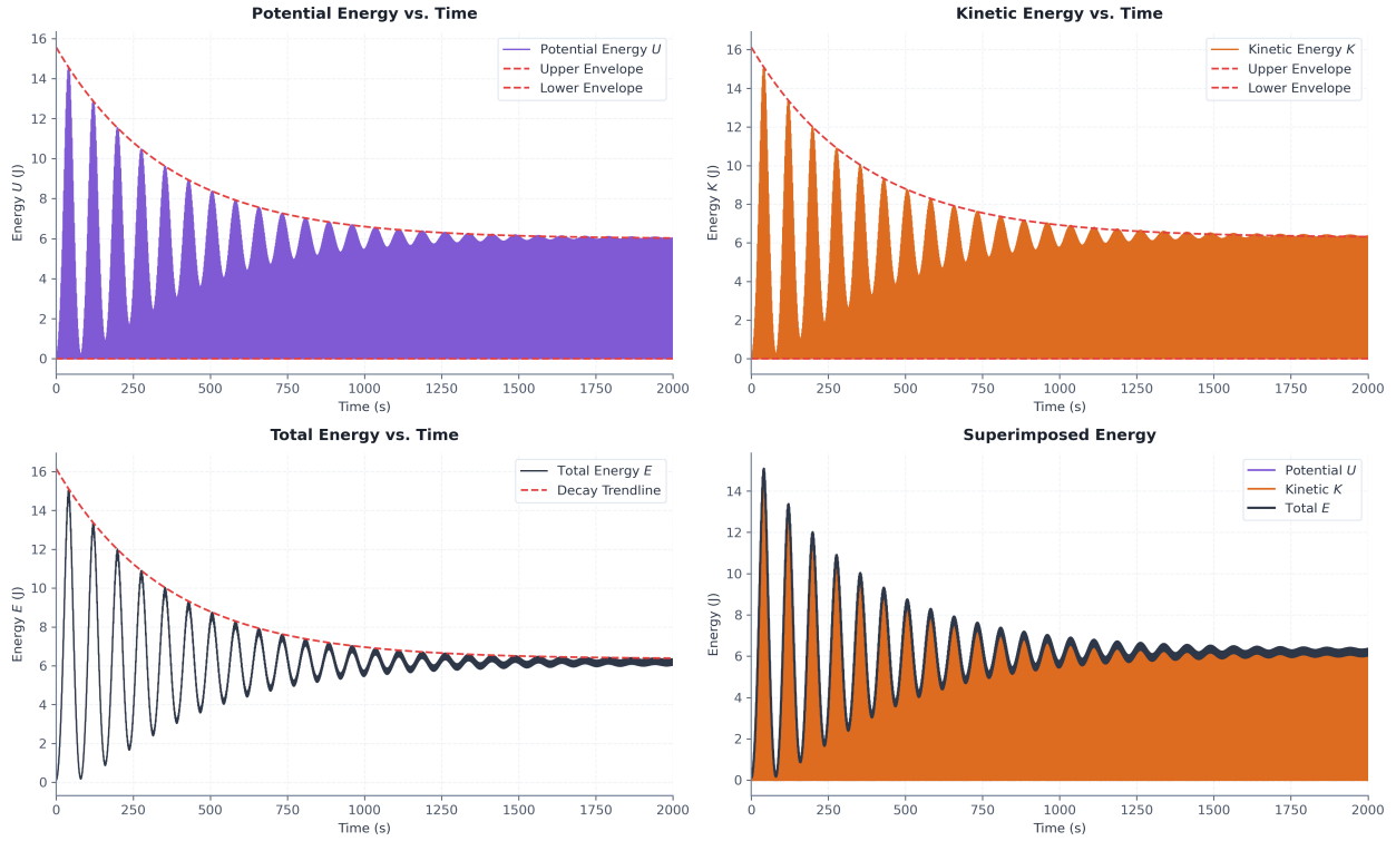
Figure 2: Potential, kinetic, and total mechanical energy as functions of time.
