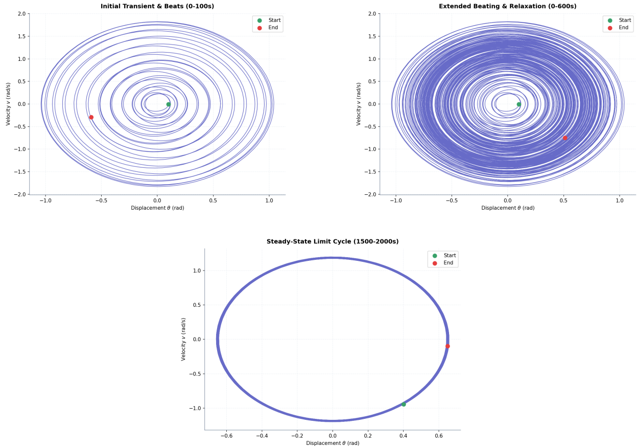
Figure 4: Phase space trajectory of the system.
